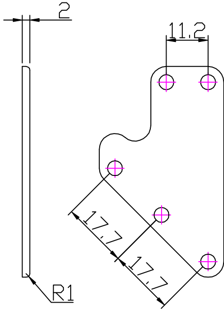
Backing Plate
